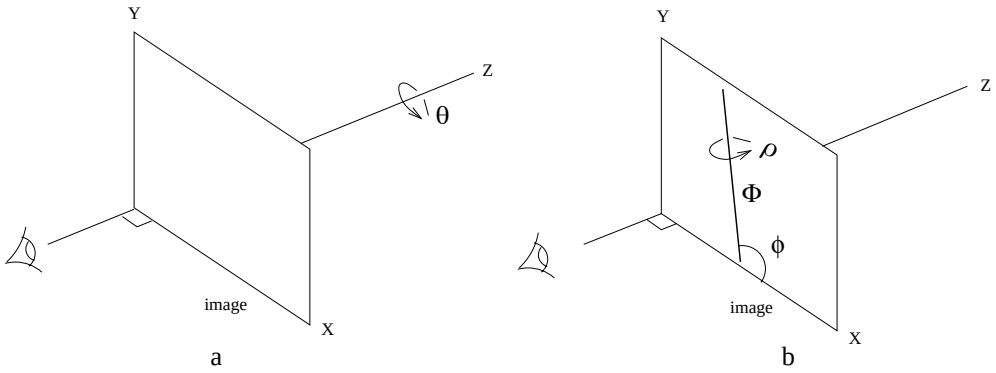
Fig. 14.10. The rotation representation. (a) rotation by \theta about the z -axis; (b) subsequent rotation by \rho about a fronto-parallel axis \Phi angled at \phi to the x -axis. The \Phi -axis has components (\cos \phi, \sin \phi, 0)^T .
