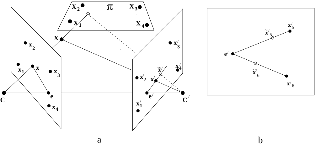
Fig. 13.9. The fundamental matrix is defined uniquely by the image of six 3D points, of which four are coplanar. (a) The parallax for one point \mathbf{X} . (b) The epipole determined by the intersection of two parallax lines: the line joining \tilde{\mathbf{x}}'_5 = H\mathbf{x}_5 to \mathbf{x}'_5 , and the join of \tilde{\mathbf{x}}'_6 = H\mathbf{x}_6 to \mathbf{x}'_6 .
