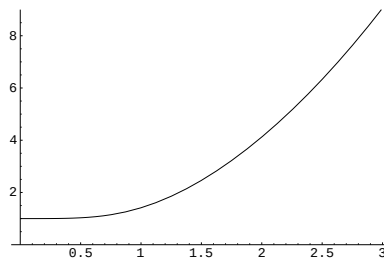
Fig. 5.5. RMS error in the position of a projected point \mathbf{x}' as a function of radial distance of \mathbf{x}' from the origin. The homography H is computed from 4 evenly spaced points on a unit circle around the origin with errors in the second image only. The RMS error is proportional to the assumed error in the points used to compute H , and the vertical axis is calibrated in terms of this assumed error.
