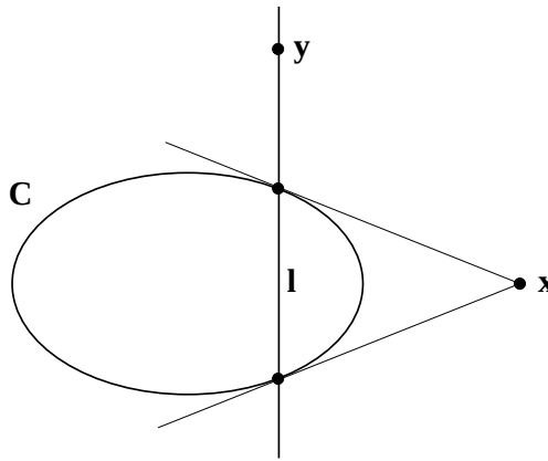
Fig. 2.19. The pole–polar relationship. The line l = Cx is the polar of the point x with respect to the conic C , and the point x = C^{-1}l is the pole of l with respect to C . The polar of x intersects the conic at the points of tangency of lines from x . If y is on l then y^T l = y^T Cx = 0 . Points x and y which satisfy y^T Cx = 0 are conjugate.
