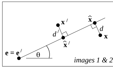
Fig. 12.9. The epipolar geometry for pure translation. In this case, corresponding epipolar lines are identical (see section 11.7.1(p293)). The epipolar line (parametrized by \theta ) that minimizes d^2 + d'^2 can be computed directly.
