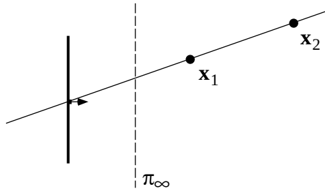
Fig. 21.4. As shown, the point x_1 is closer to the camera than x_2 . However, if an orientation-reversing projectivity is applied, taking \pi_\infty to infinity, then both x_1 and x_2 remain in front of the camera, but x_2 is closer to the camera than x_1 .
