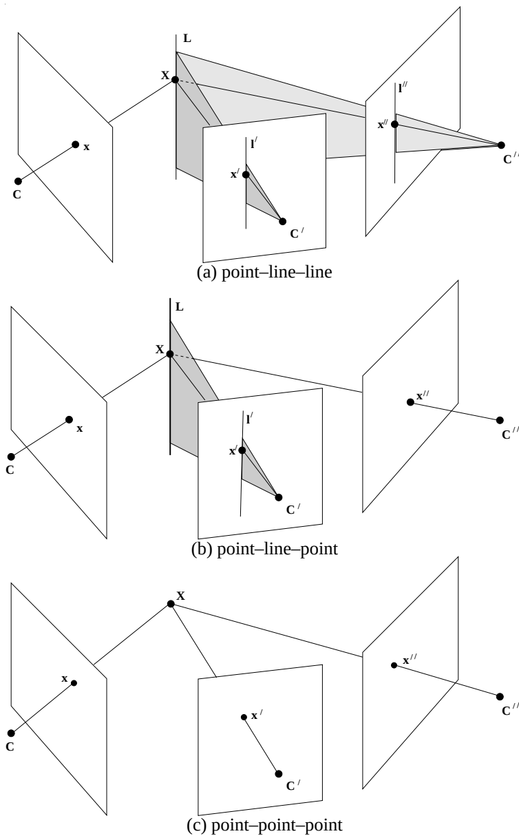
Fig. 15.4. Incidence relations. (a) Consider a 3-view point correspondence x \leftrightarrow x' \leftrightarrow x'' . If l' and l'' are any two lines through x' and x'' respectively, then x \leftrightarrow l' \leftrightarrow l'' forms a point-line-line correspondence, corresponding to a 3D line L . Consequently, (15.5) holds for any choice of lines l' through x' and l'' through x'' . (b) The space point X is incident with the space line L . This defines an incidence relation x \leftrightarrow l' \leftrightarrow x'' between their images. (c) The correspondence x \leftrightarrow x' \leftrightarrow x'' arising from the image of a space point X .
