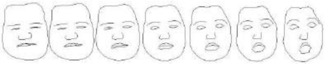
Fig. 18.1. Shape basis. A face template is represented by N equally spaced 2D points (here N = 140 ). The central face of the seven is the mean shape and the faces to the left or right are generated by adding or subtracting, respectively, the basis shape that accounts for the maximum variation in the training set. In this case the basis spans expressions from surprised to disgruntled. Facial expressions are learnt by tracking the face of an actor with the template whilst he changes expression but does not vary his head pose. Each frame of the training sequence generates a set of N 2D points, and the coordinates of these are rewritten as a 2N -vector. A 2N \times f matrix is then composed from these vectors, where f is the number of training frames, and the basis shapes are computed from the singular vectors of this matrix. Figure courtesy of Richard Bowden.
