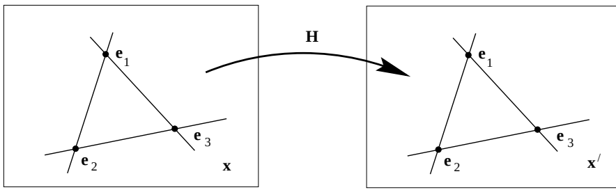
Fig. 2.21. Fixed points and lines of a plane projective transformation. There are three fixed points, and three fixed lines through these points. The fixed lines and points may be complex. Algebraically, the fixed points are the eigenvectors, \mathbf{e}_i , of the point transformation ( \mathbf{x}' = \mathbf{H}\mathbf{x} ), and the fixed lines are eigenvectors of the line transformation ( \mathbf{l}' = \mathbf{H}^{-T}\mathbf{l} ). Note, the fixed line is not fixed pointwise: under the transformation, points on the line are mapped to other points on the line; only the fixed points are mapped to themselves.
