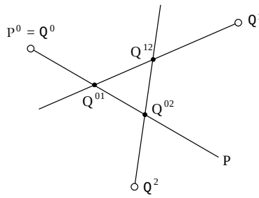
Fig. 22.7. Configuration of the three camera centres and the three ambiguous points. If the three points Q^{ij} are distinct, then they all lie in the plane of the camera centres C_Q^i .
