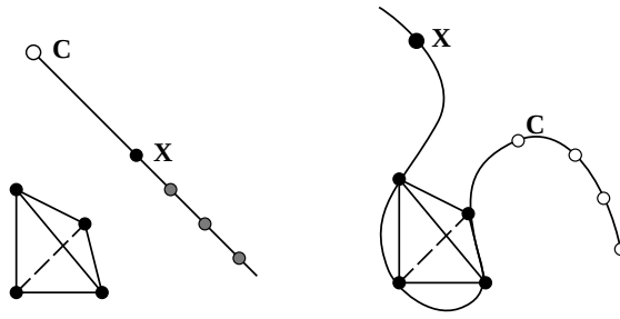
Fig. 22.5. Left: Any point on the line passing through C and X is projected to the same point from projection centre C . Right: The dual statement – from any centre of projection C lying on a twisted cubic passing through X and the vertices of the reference tetrahedron, the five points are projected in the same way (up to projective equivalence). Thus a camera is constrained to lie on a twisted cubic by its image of five known points.
