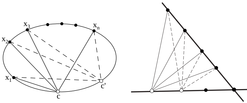
Fig. 22.2. The points x_1, \dots, x_n project in equivalent ways to the two camera centres c and c' .
