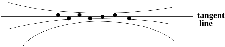
Fig. 11.7. Estimating a conic from point data (shown as •) may be poorly conditioned. All of the conics shown have residuals within the point error distribution. However, even though there is ambiguity in the estimated conic, the tangent line is well defined, and can be computed from the points.
